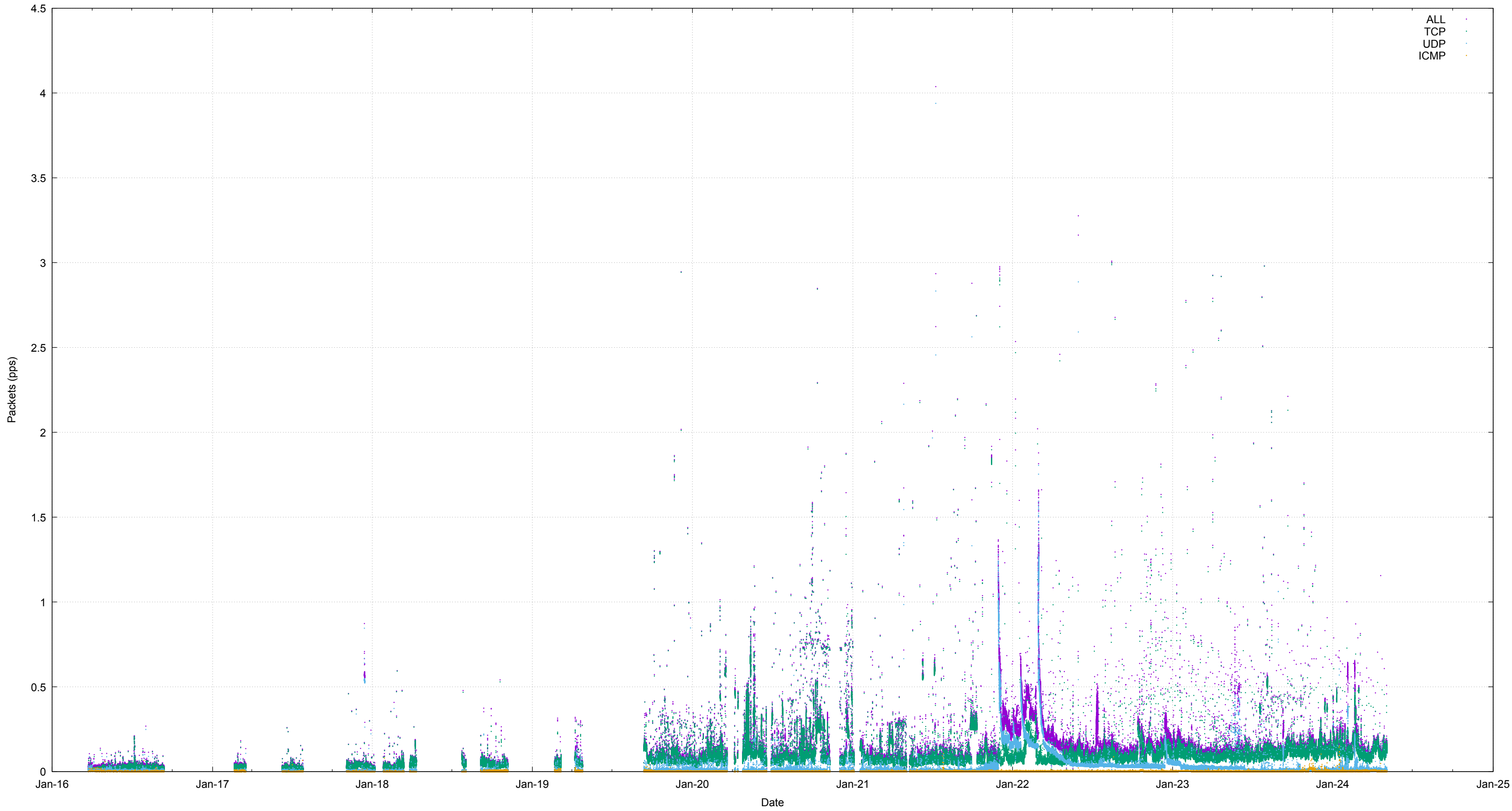
Average Packet Rate per /32 address (pps) (log scale)
