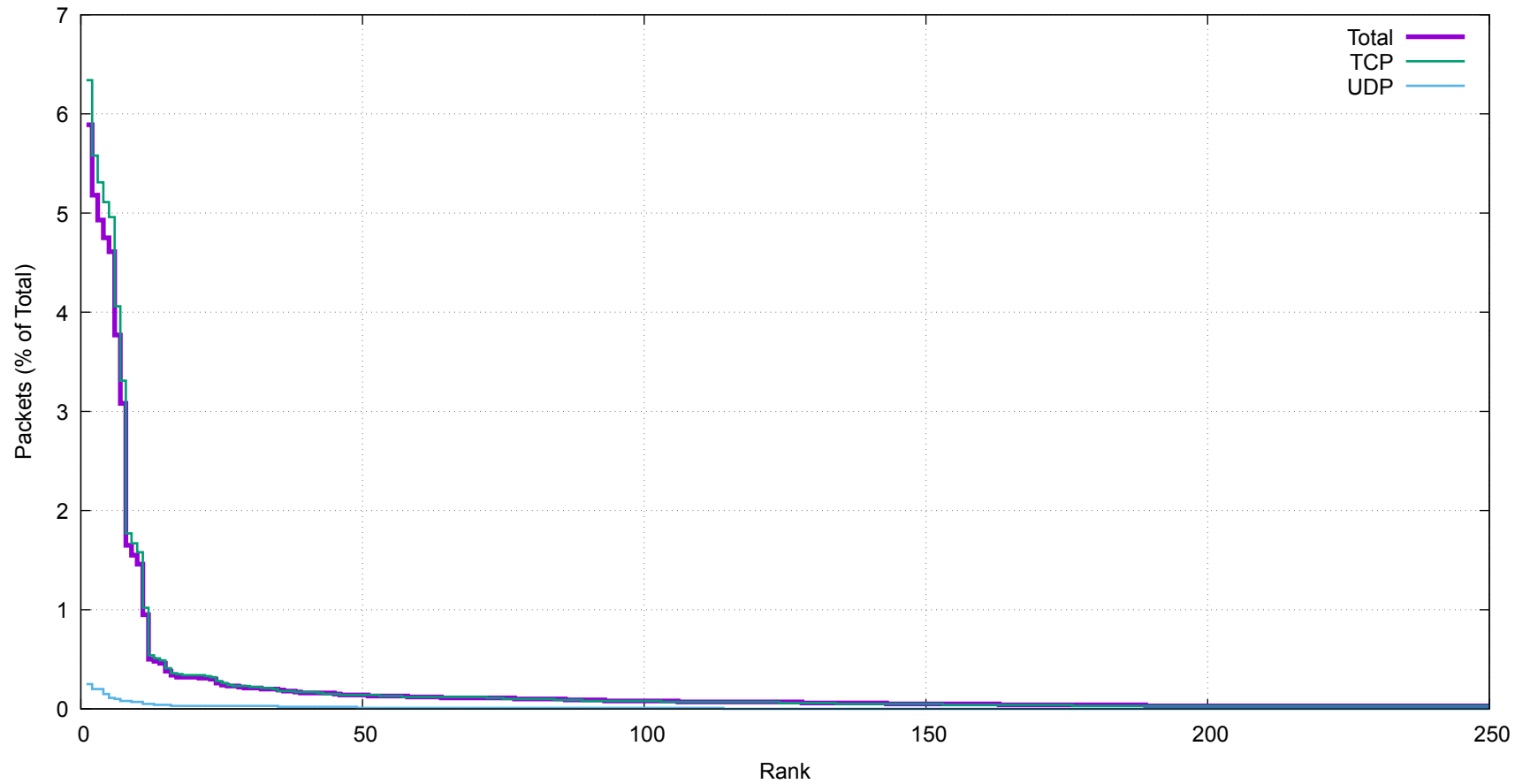
8-Day Top Source Addresses
